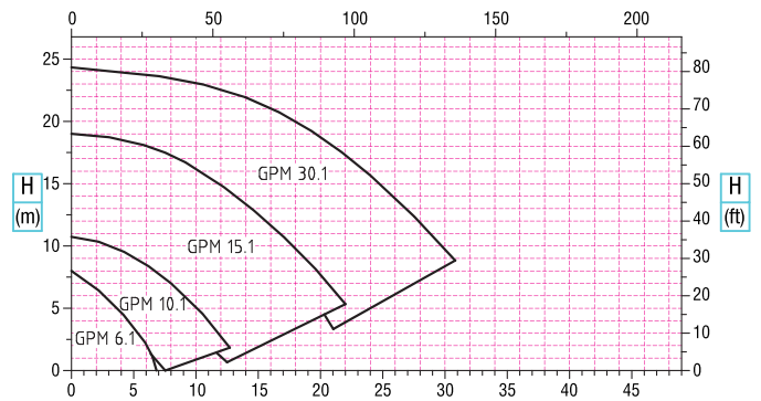
Q (m³/h) GPM. 1 SS316 3500 rpm
